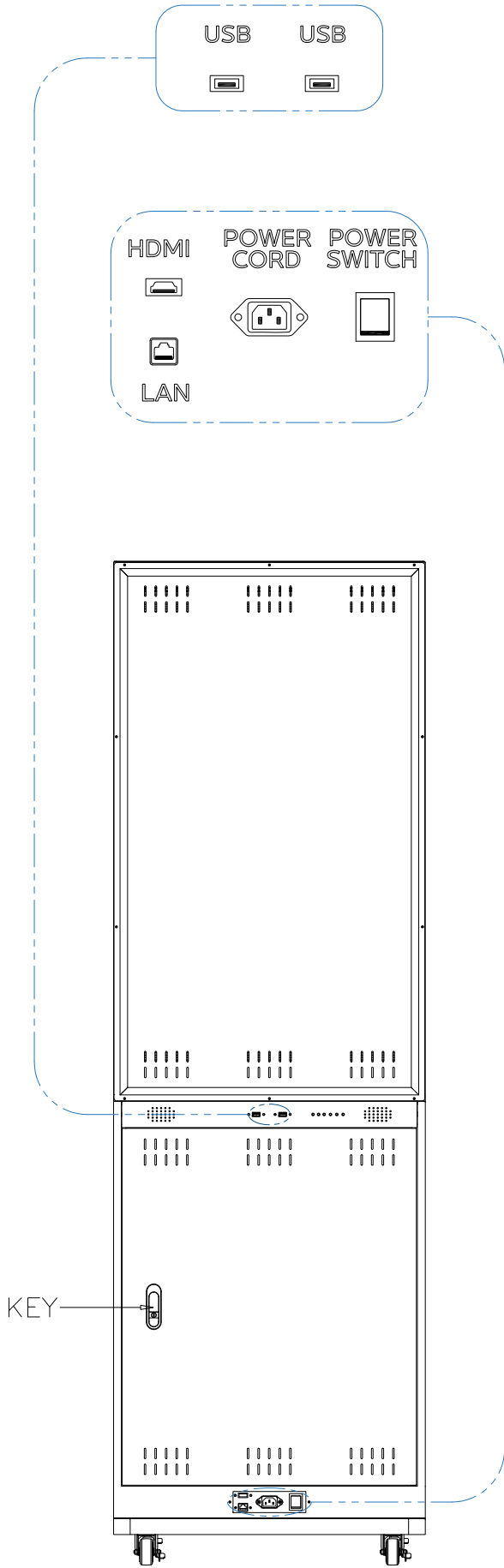
REAR VIEW
