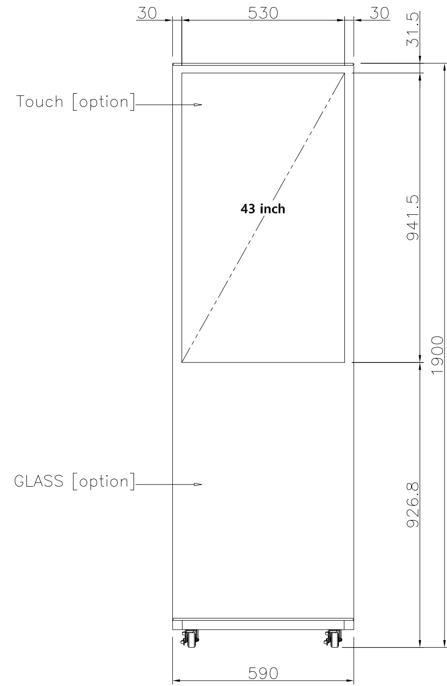
FRONT VIEW
