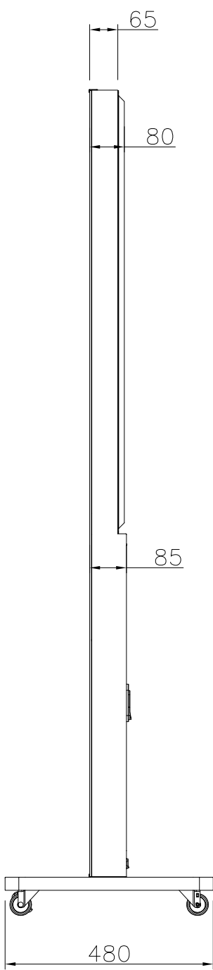
SIDE VIEW
